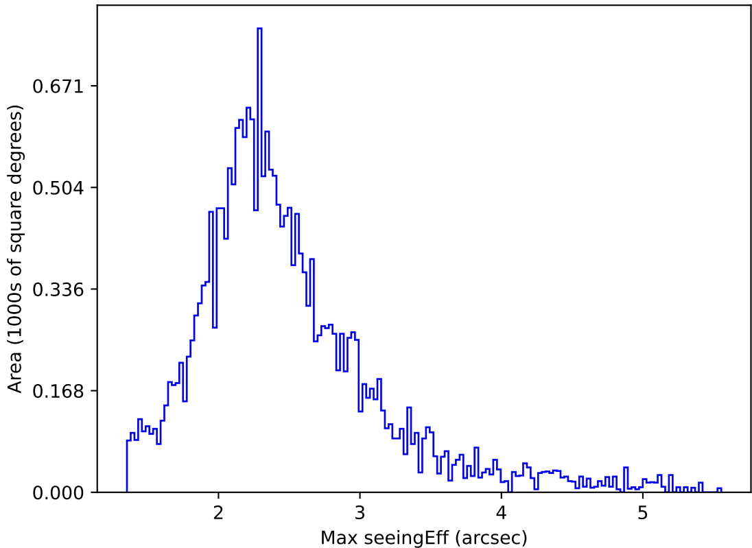
weather_cloudso36v3.4_10yrs All sky y band: Max seeingEff
