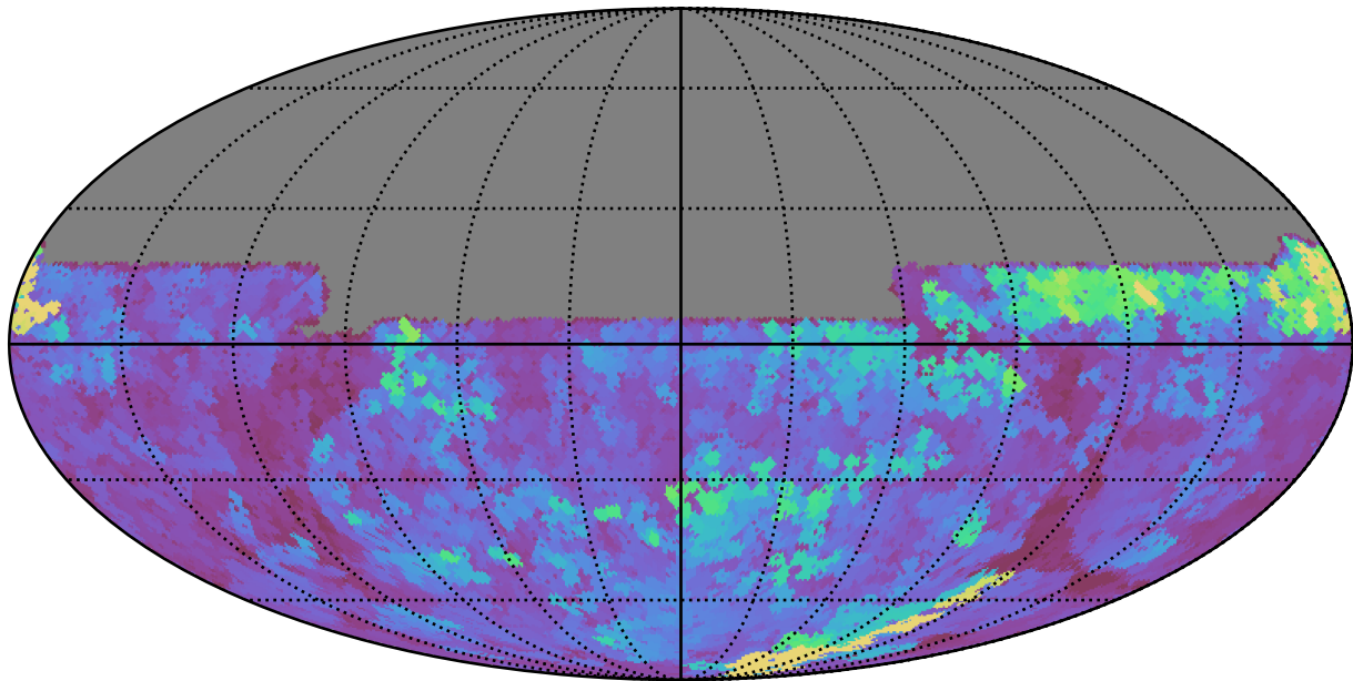
weather_cloudso36v3.4_10yrs All sky u band: Max seeingEff
