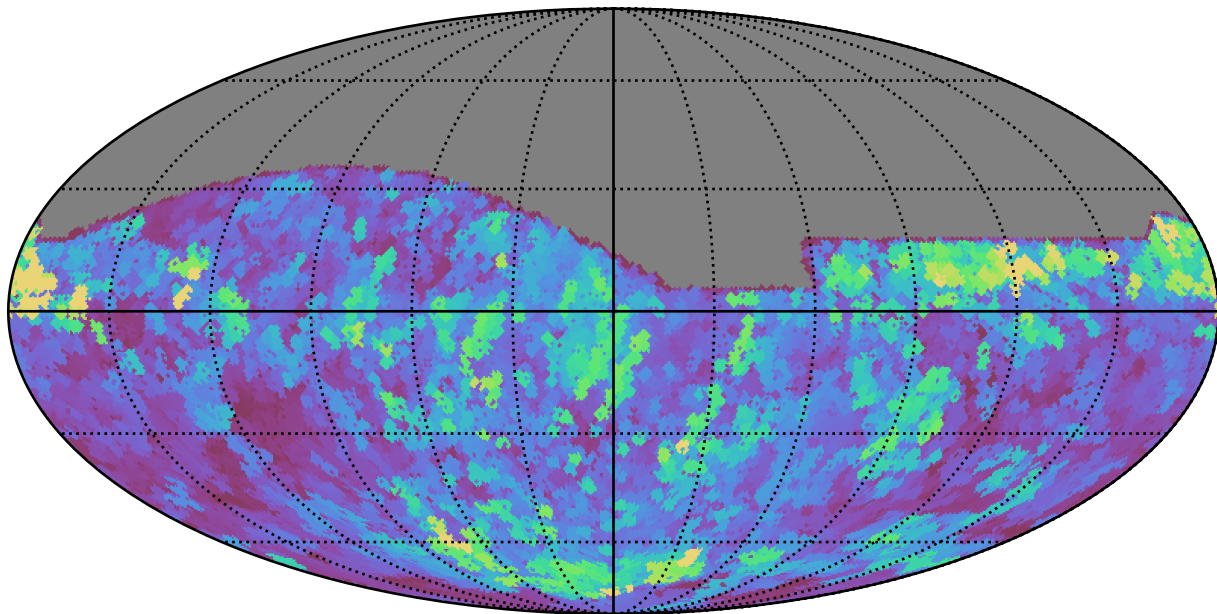
weather_cloudso36v3.4_10yrs All sky r band: Max seeingEff
