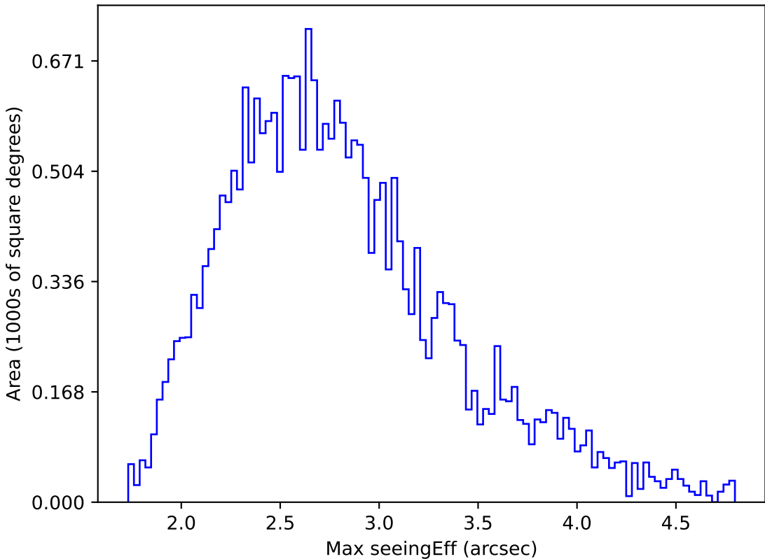
weather_cloudso36v3.4_10yrs All sky r band: Max seeingEff
