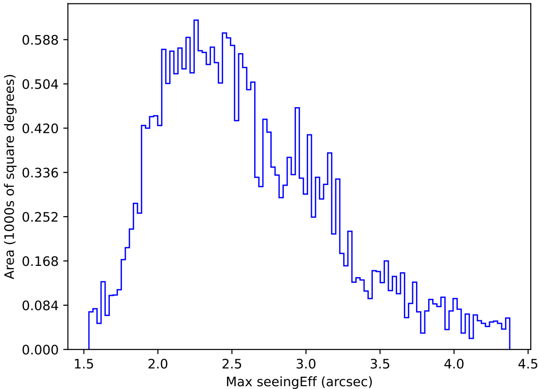
weather_cloudso36v3.4_10yrs All sky g band: Max seeingEff
