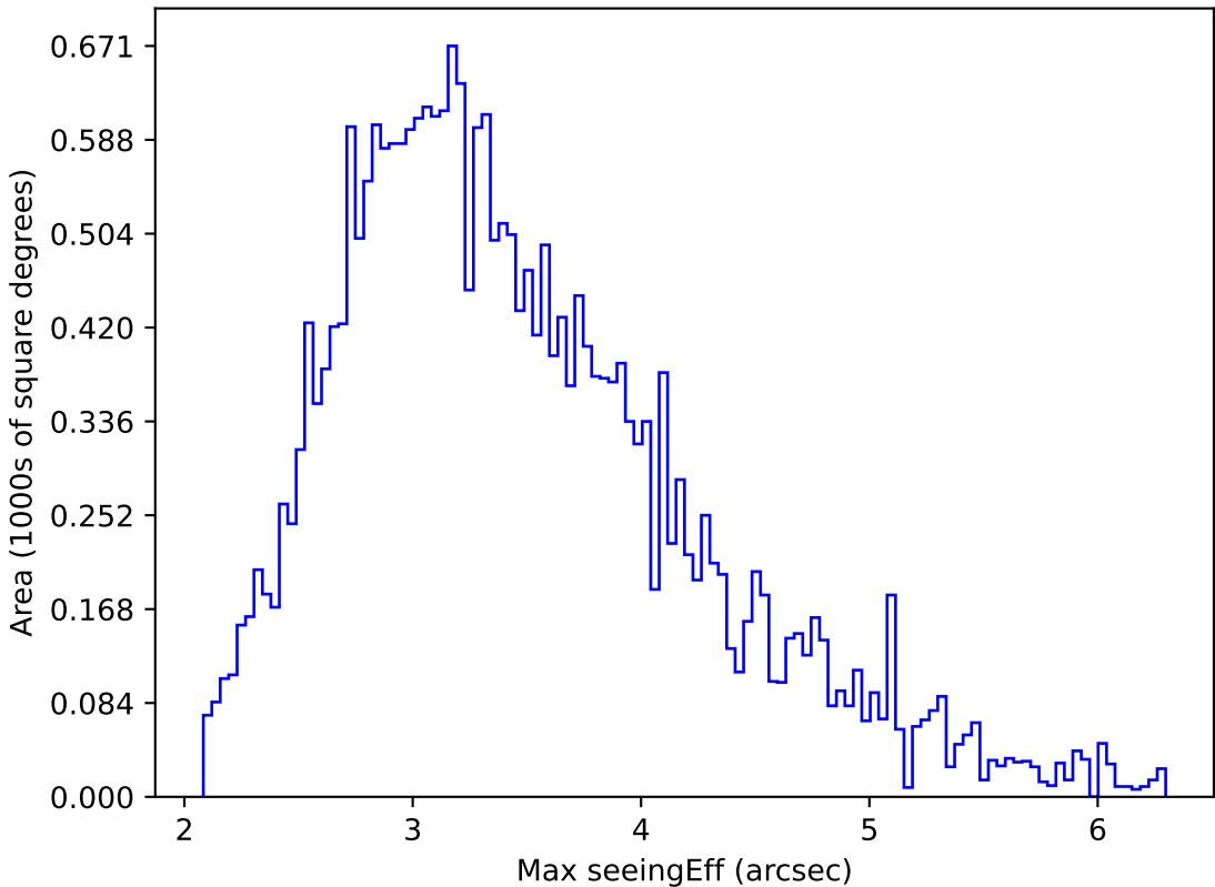
weather_cloudso36v3.4_10yrs All sky all bands: Max seeingEff
