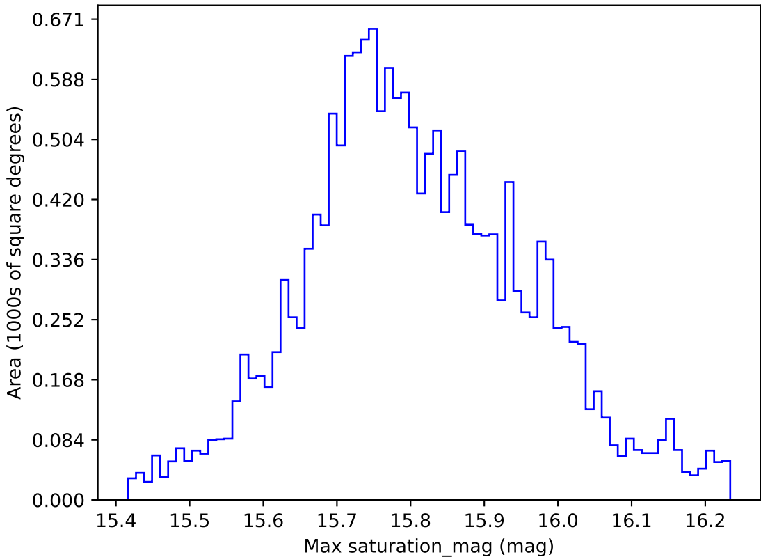
weather_cloudso36v3.4_10yrs WFD all bands: Max saturation_mag
