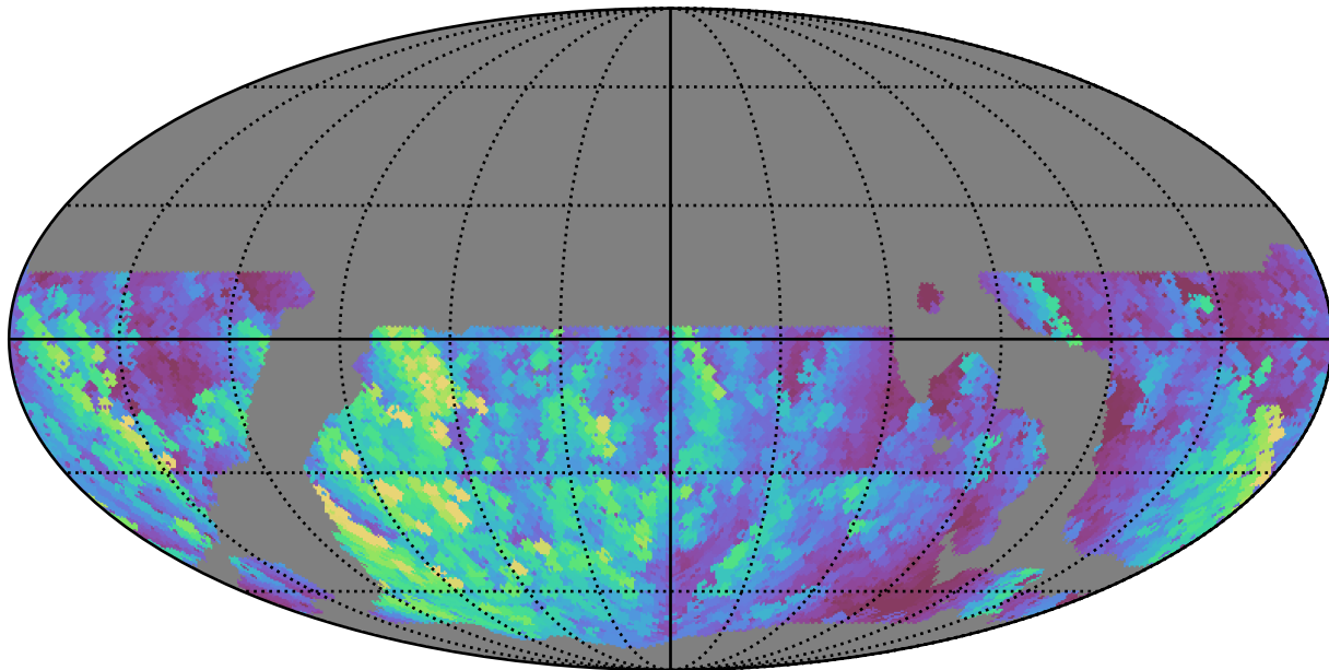
weather_cloudso36v3.4_10yrs WFD u band: Max normairmass
