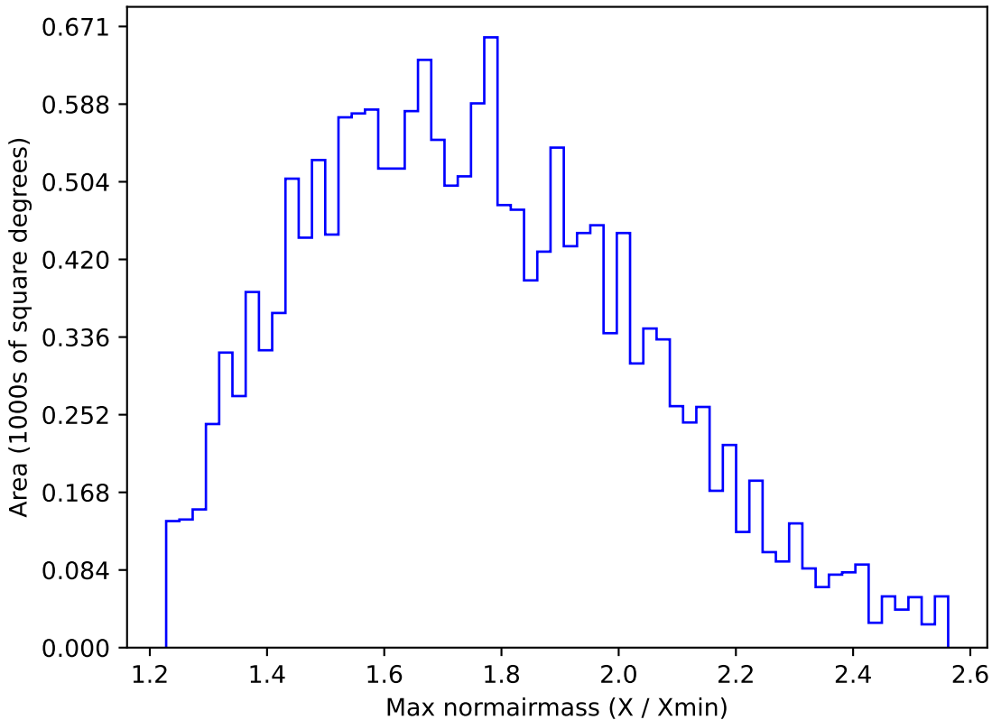
weather_cloudso36v3.4_10yrs WFD u band: Max normairmass
