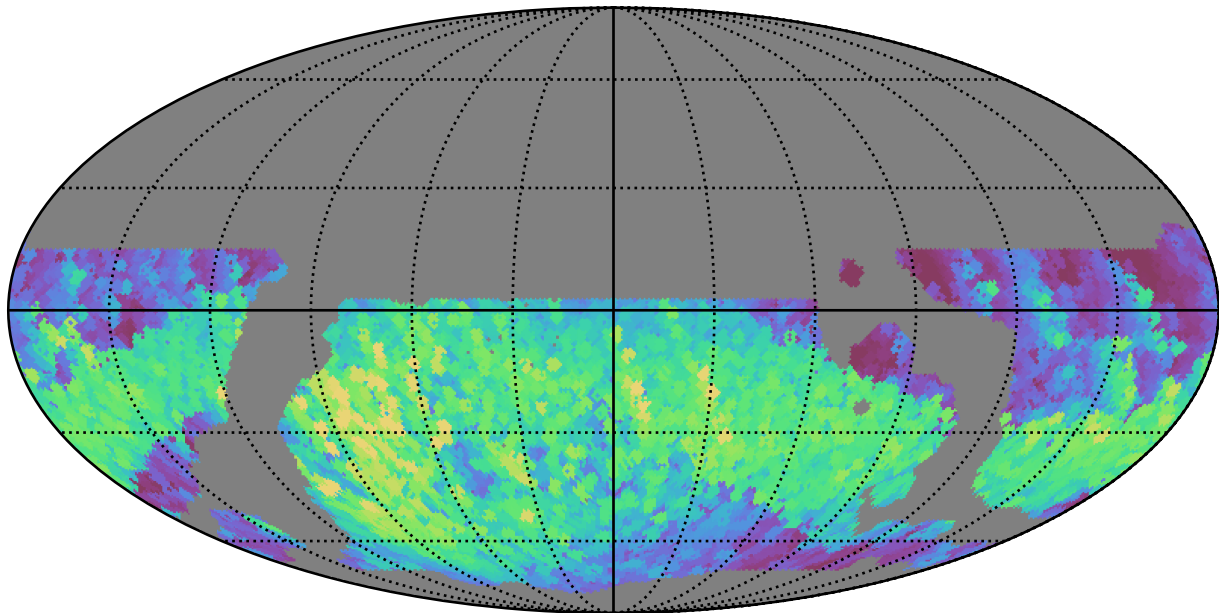
weather_cloudso36v3.4_10yrs WFD r band: Max normairmass
