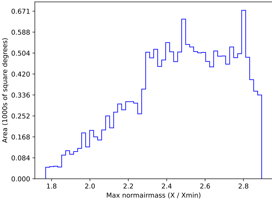
weather_cloudso36v3.4_10yrs WFD all bands: Max normairmass
