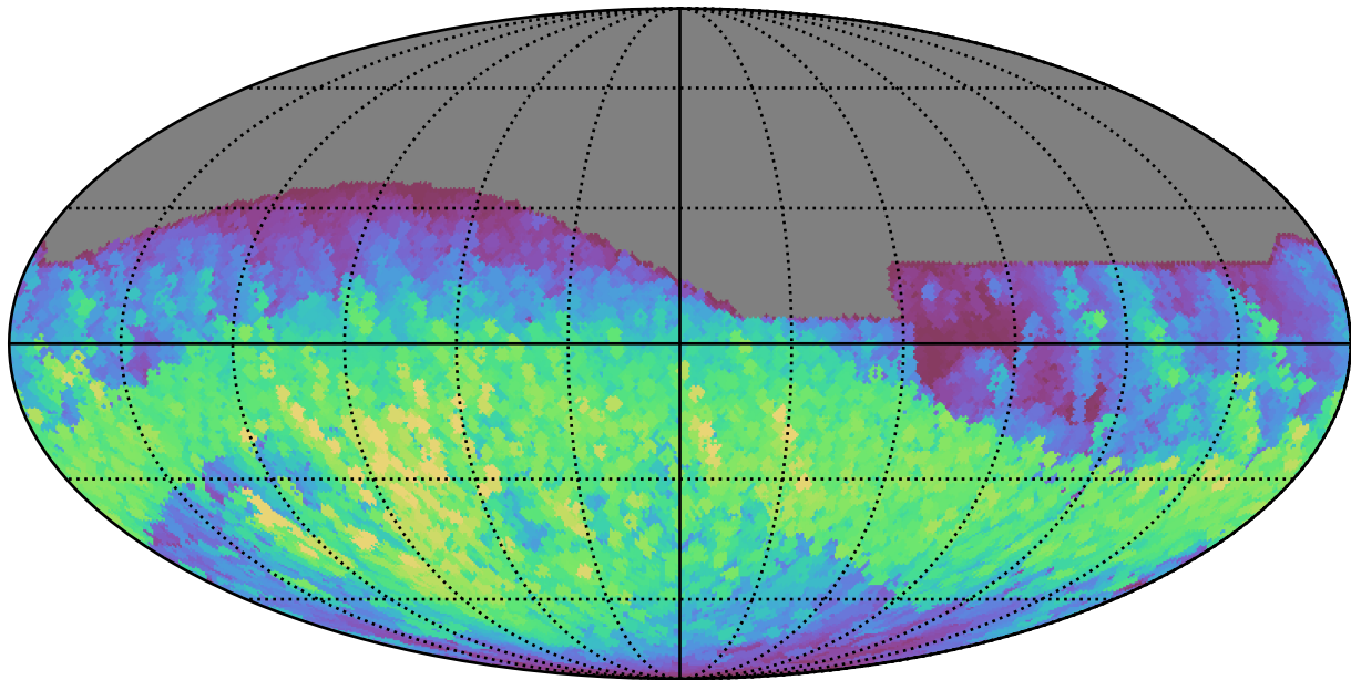
weather_cloudso36v3.4_10yrs All sky r band: Max normairmass
