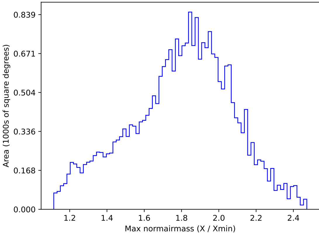
weather_cloudso36v3.4_10yrs All sky g band: Max normairmass
