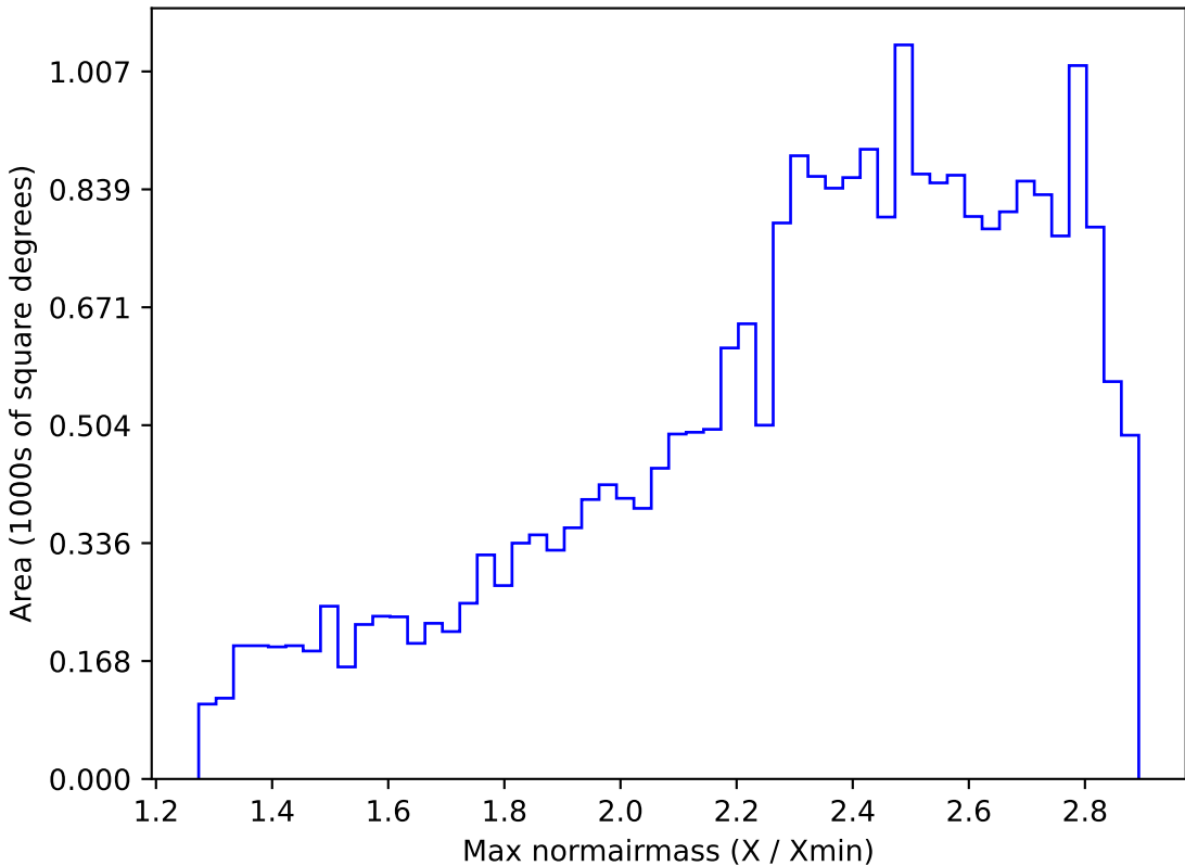
weather_cloudso36v3.4_10yrs All sky all bands: Max normairmass
