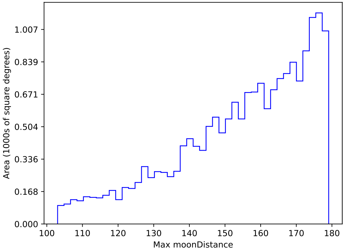
weather_cloudso36v3.4_10yrs WFD z band: Max moonDistance
