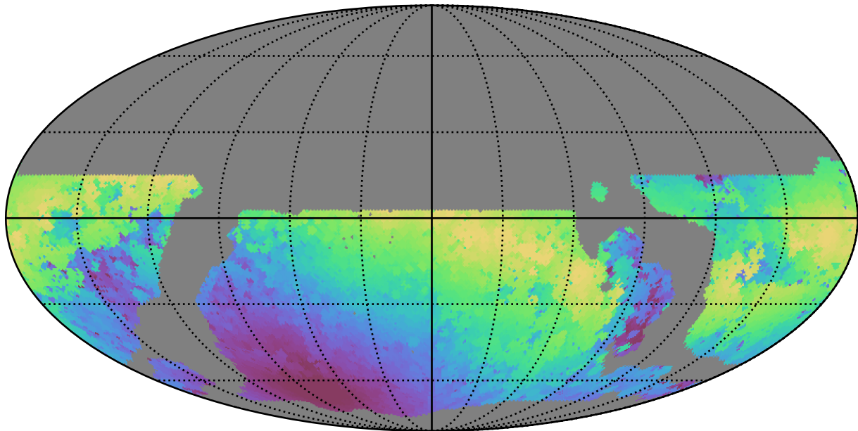
weather_cloudso36v3.4_10yrs WFD y band: Max moonDistance
