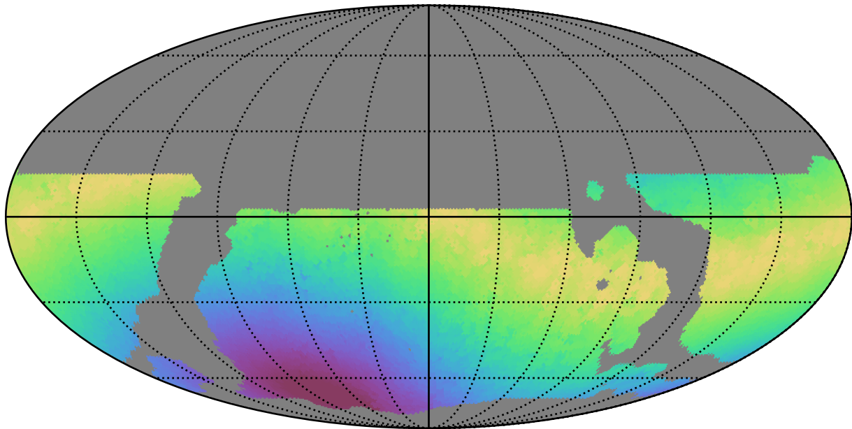
weather_cloudso36v3.4_10yrs WFD u band: Max moonDistance
