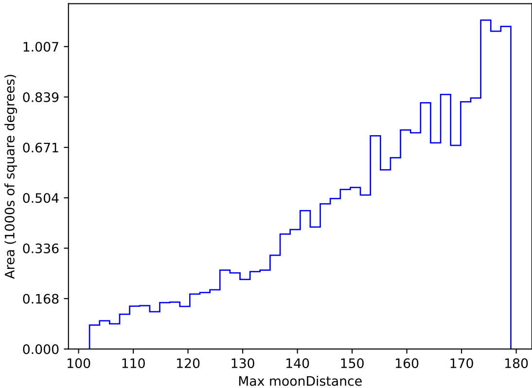
weather_cloudso36v3.4_10yrs WFD u band: Max moonDistance
