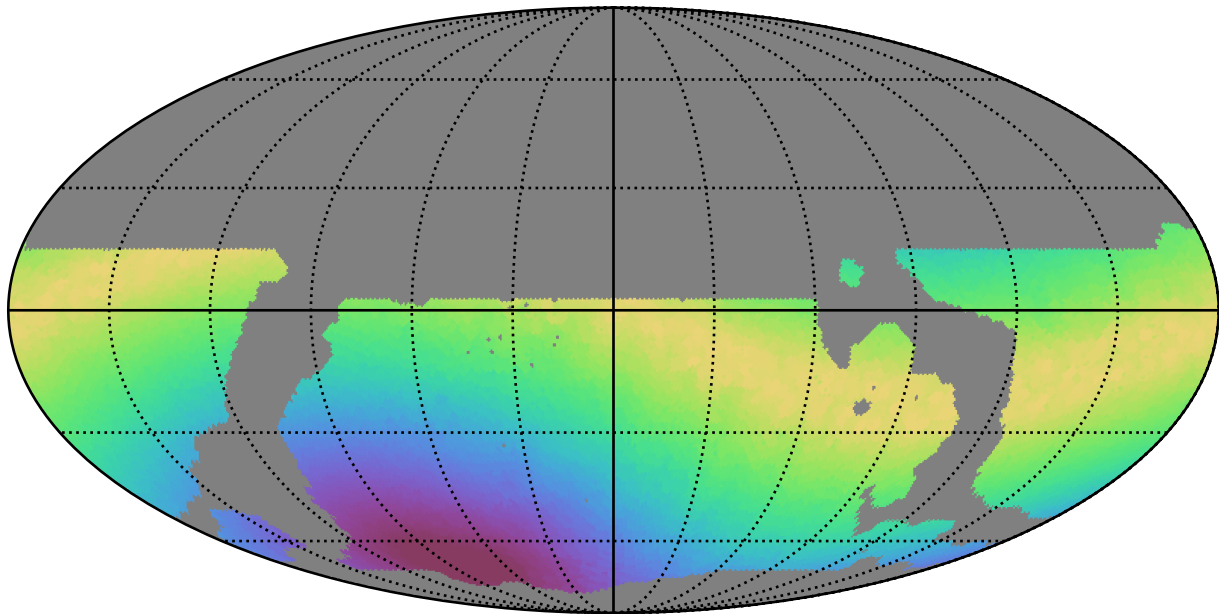
weather_cloudso36v3.4_10yrs WFD r band: Max moonDistance
