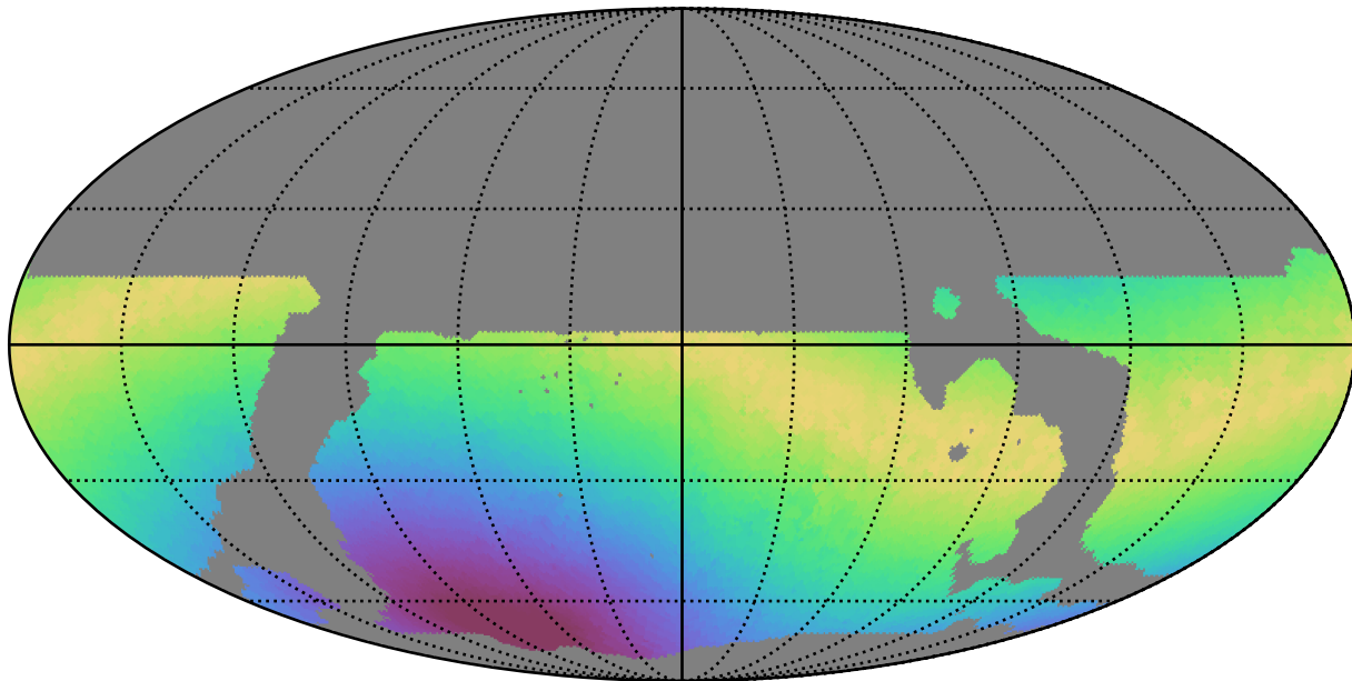
weather_cloudso36v3.4_10yrs WFD i band: Max moonDistance
