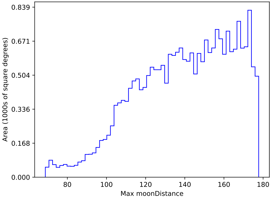
weather_cloudso36v3.4_10yrs All sky y band: Max moonDistance
