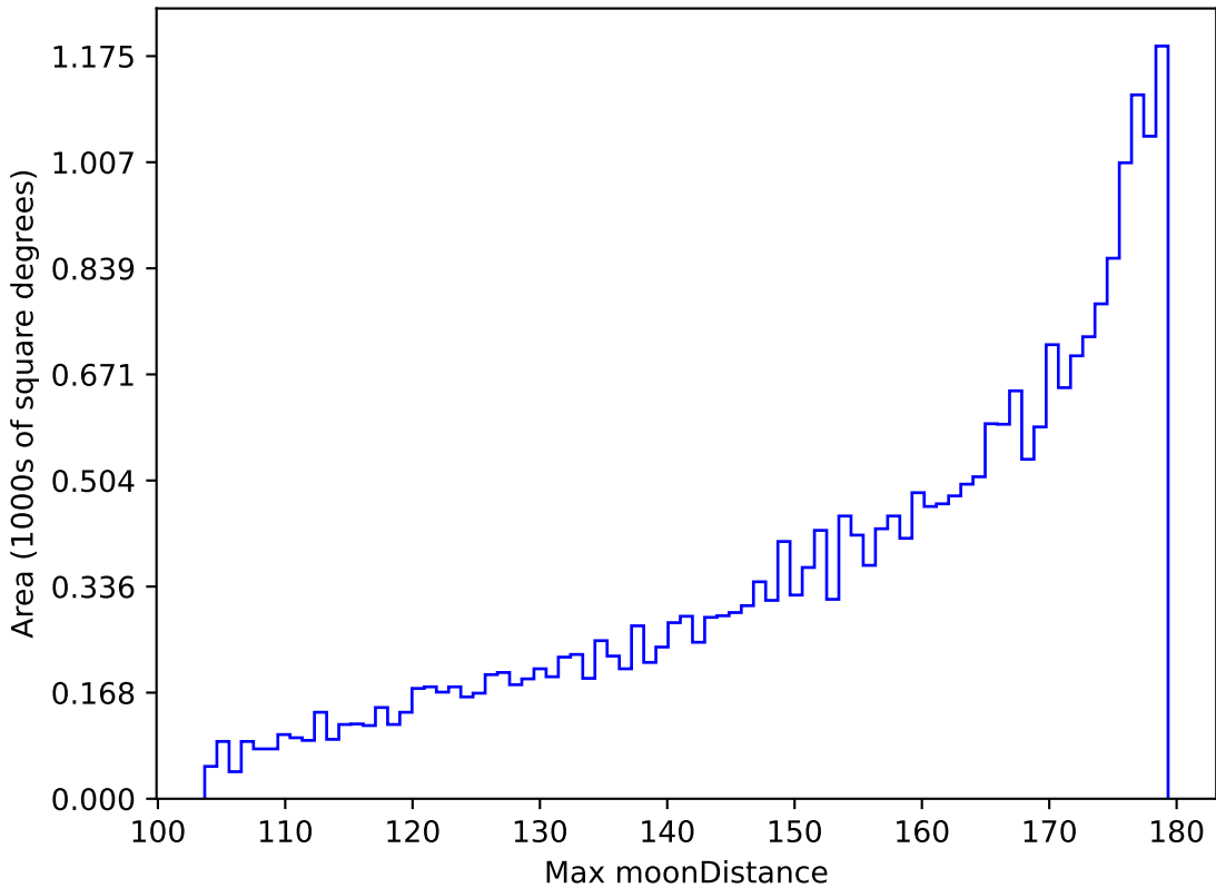
weather_cloudso36v3.4_10yrs All sky r band: Max moonDistance
