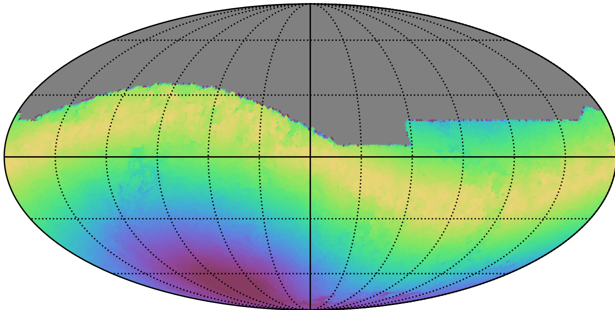
weather_cloudso36v3.4_10yrs All sky i band: Max moonDistance
