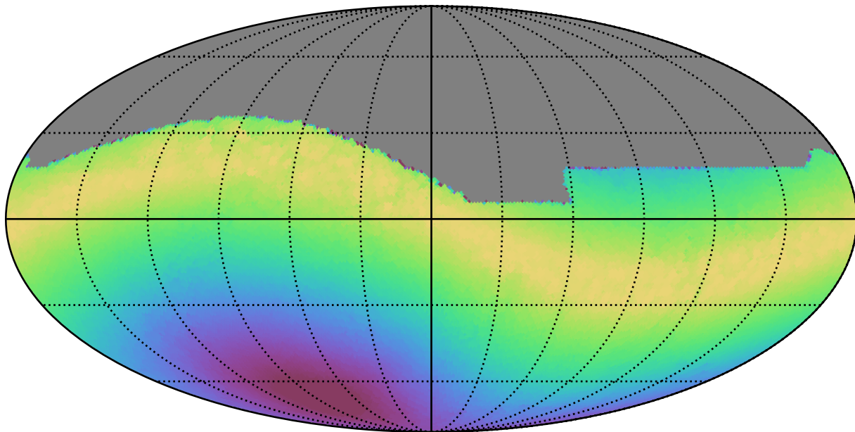
weather_cloudso36v3.4_10yrs All sky all bands: Max moonDistance
