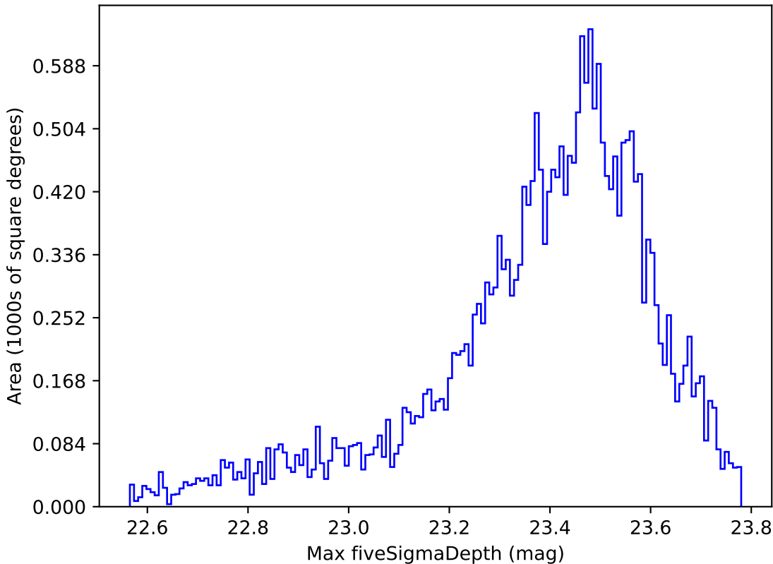
weather_cloudso36v3.4_10yrs Yr 1 z band: Max fiveSigmaDepth
