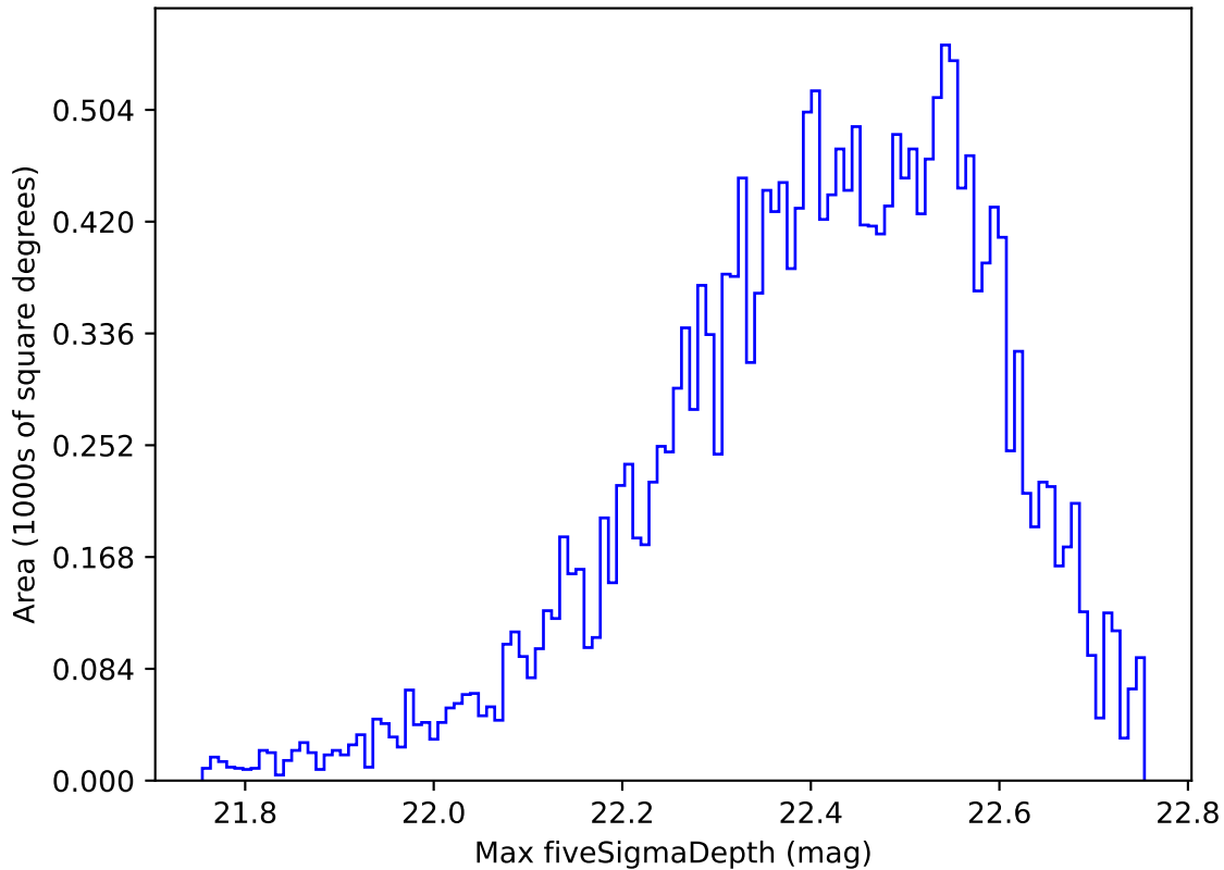
weather_cloudso36v3.4_10yrs Yr 1 y band: Max fiveSigmaDepth
