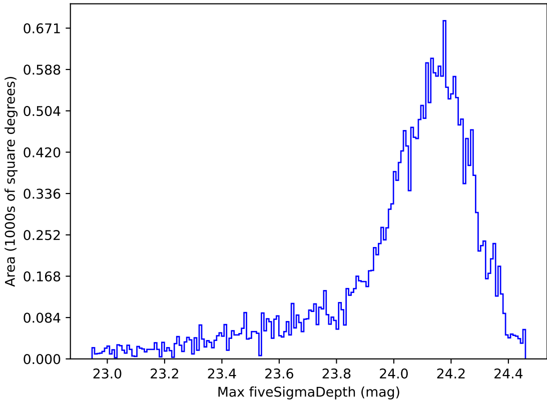
weather_cloudso36v3.4_10yrs Yr 1 i band: Max fiveSigmaDepth
