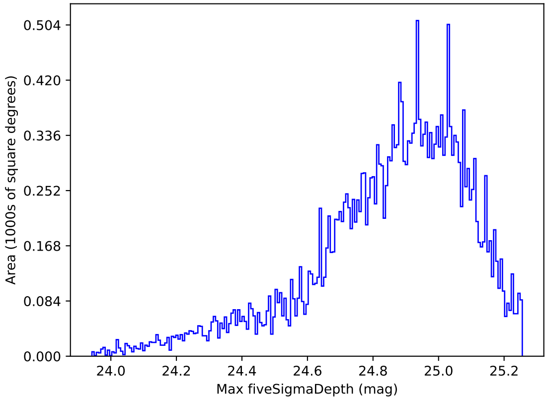
weather_cloudso36v3.4_10yrs Yr 1 all bands: Max fiveSigmaDepth
