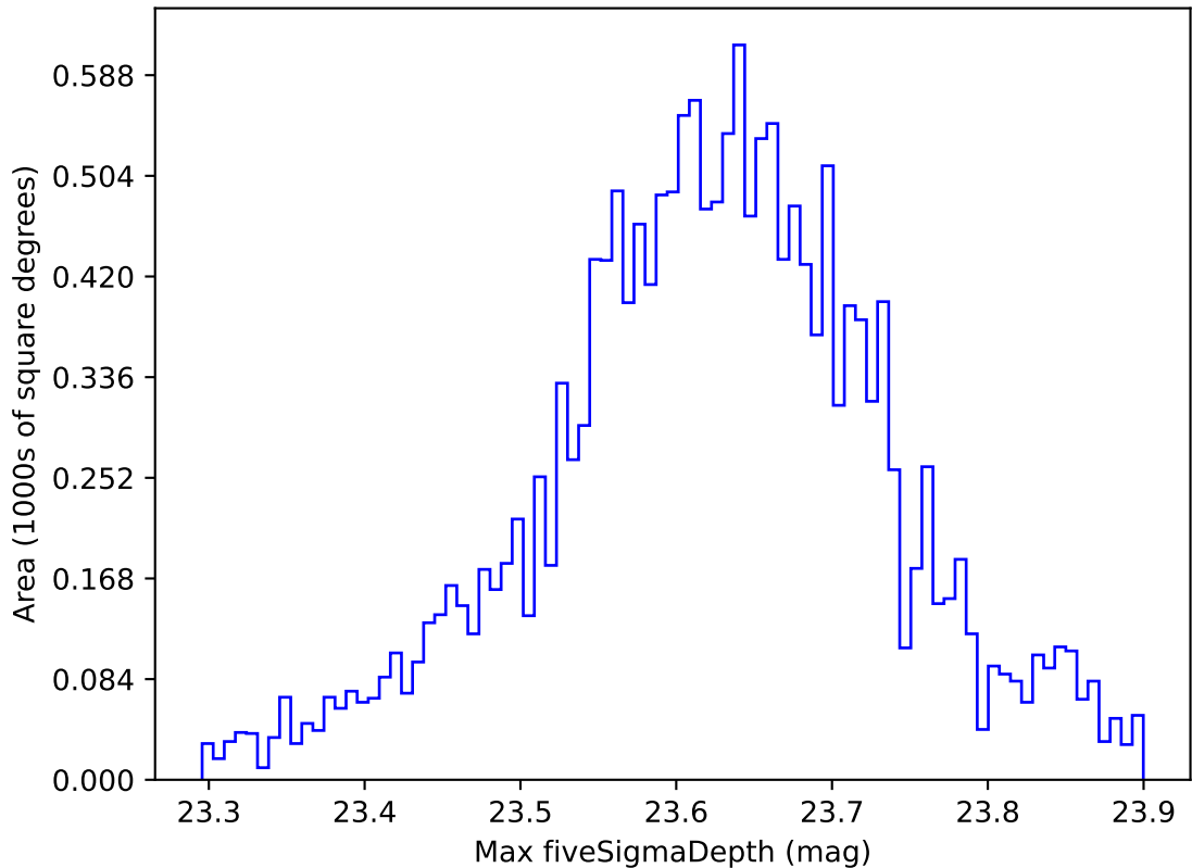
weather_cloudso36v3.4_10yrs WFD z band: Max fiveSigmaDepth
