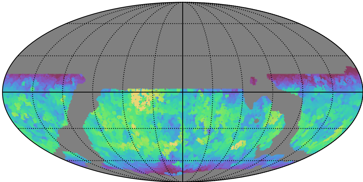
weather_cloudso36v3.4_10yrs WFD y band: Max fiveSigmaDepth
