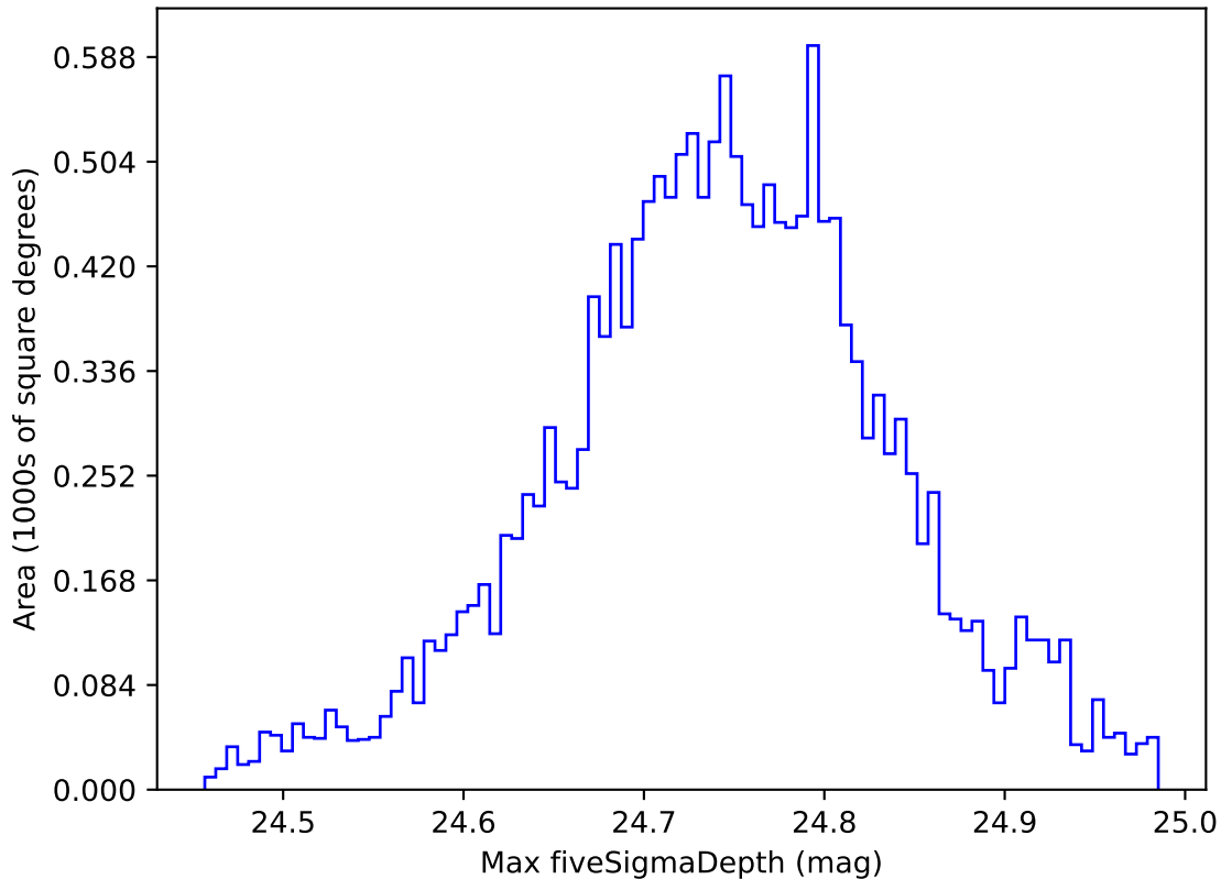
weather_cloudso36v3.4_10yrs WFD r band: Max fiveSigmaDepth
