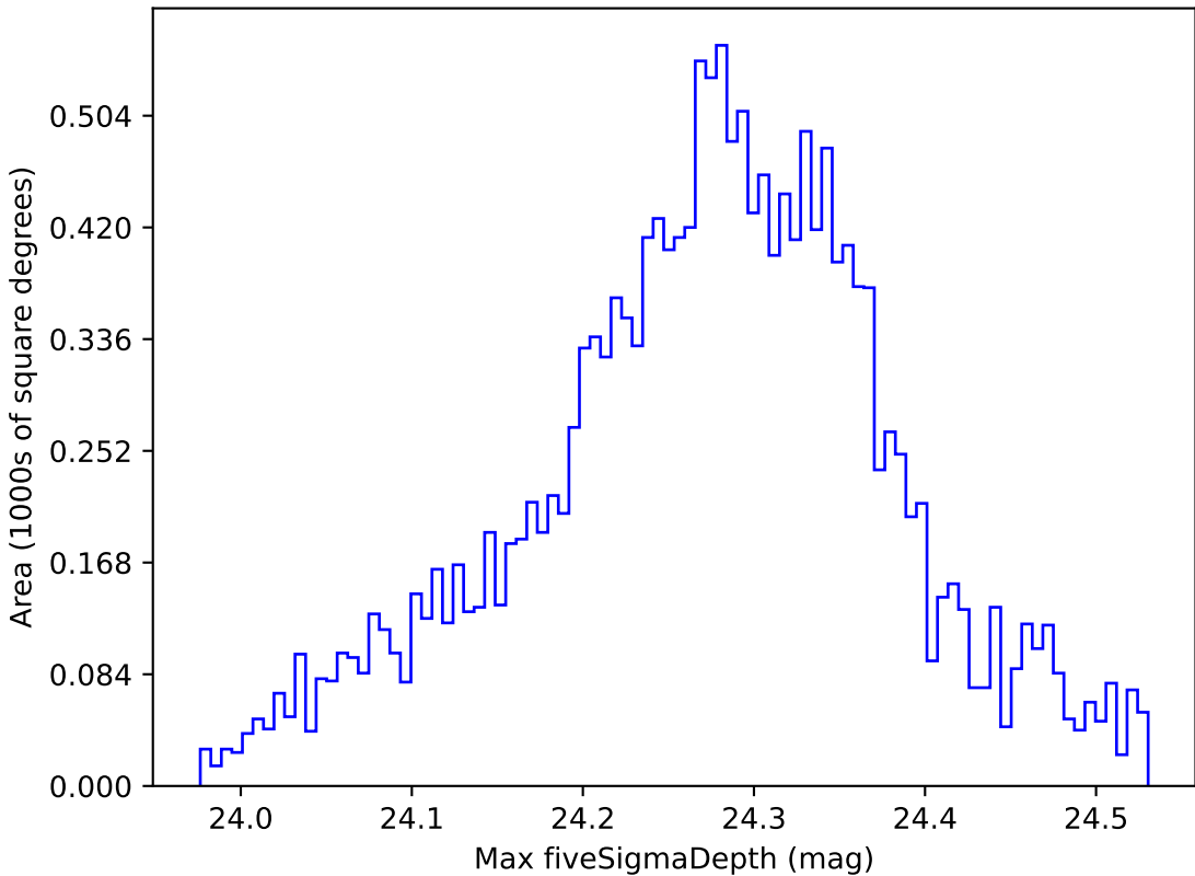
weather_cloudso36v3.4_10yrs WFD i band: Max fiveSigmaDepth
