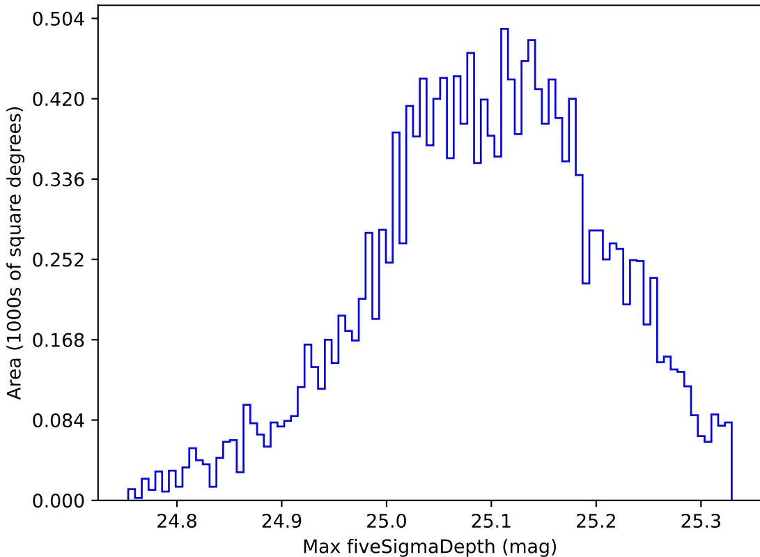
weather_cloudso36v3.4_10yrs WFD g band: Max fiveSigmaDepth
