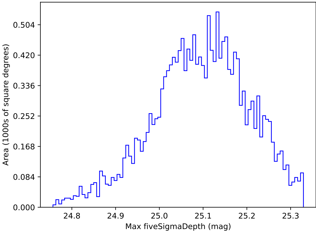
weather_cloudso36v3.4_10yrs WFD all bands: Max fiveSigmaDepth
