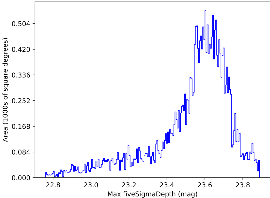
weather_cloudso36v3.4_10yrs All sky z band: Max fiveSigmaDepth
