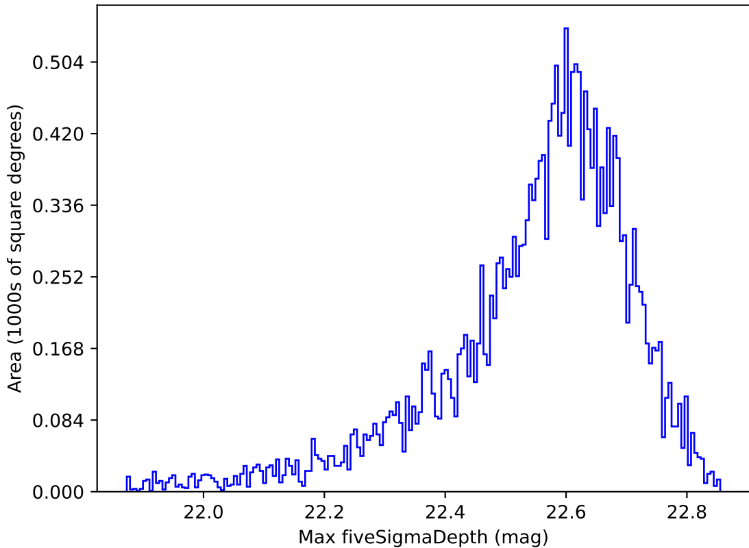
weather_cloudso36v3.4_10yrs All sky y band: Max fiveSigmaDepth
