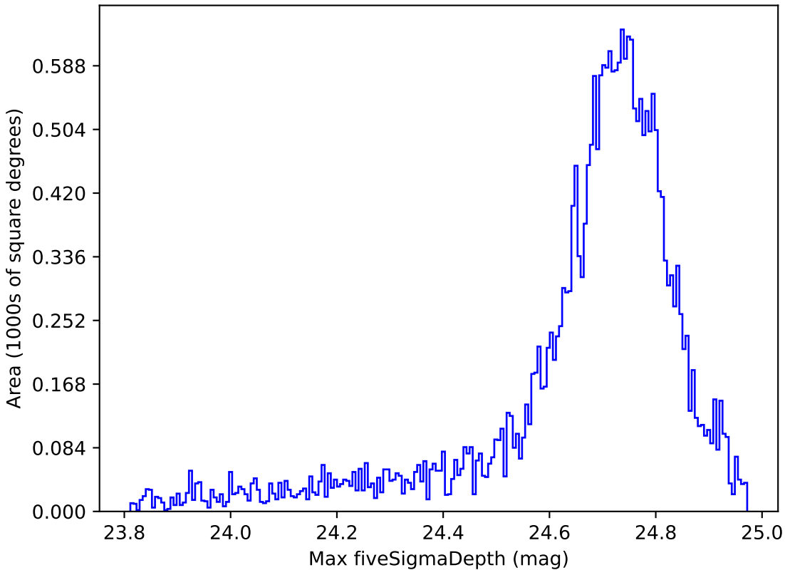
weather_cloudso36v3.4_10yrs All sky r band: Max fiveSigmaDepth
