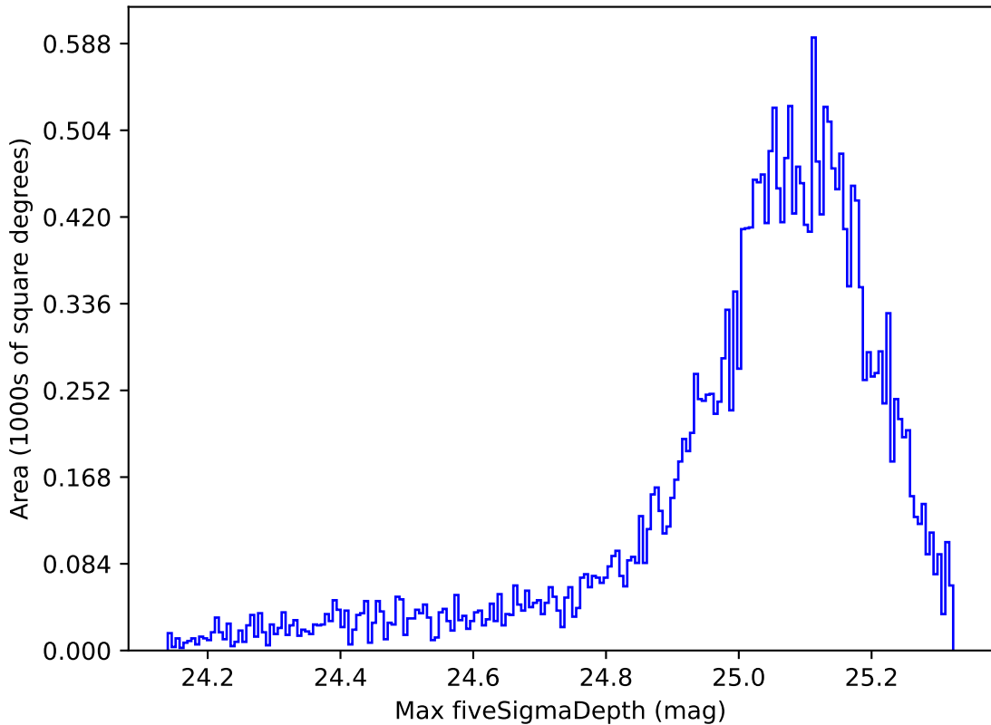
weather_cloudso36v3.4_10yrs All sky g band: Max fiveSigmaDepth
