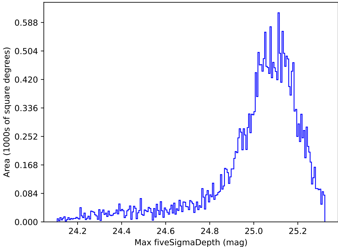
weather_cloudso36v3.4_10yrs All sky all bands: Max fiveSigmaDepth
