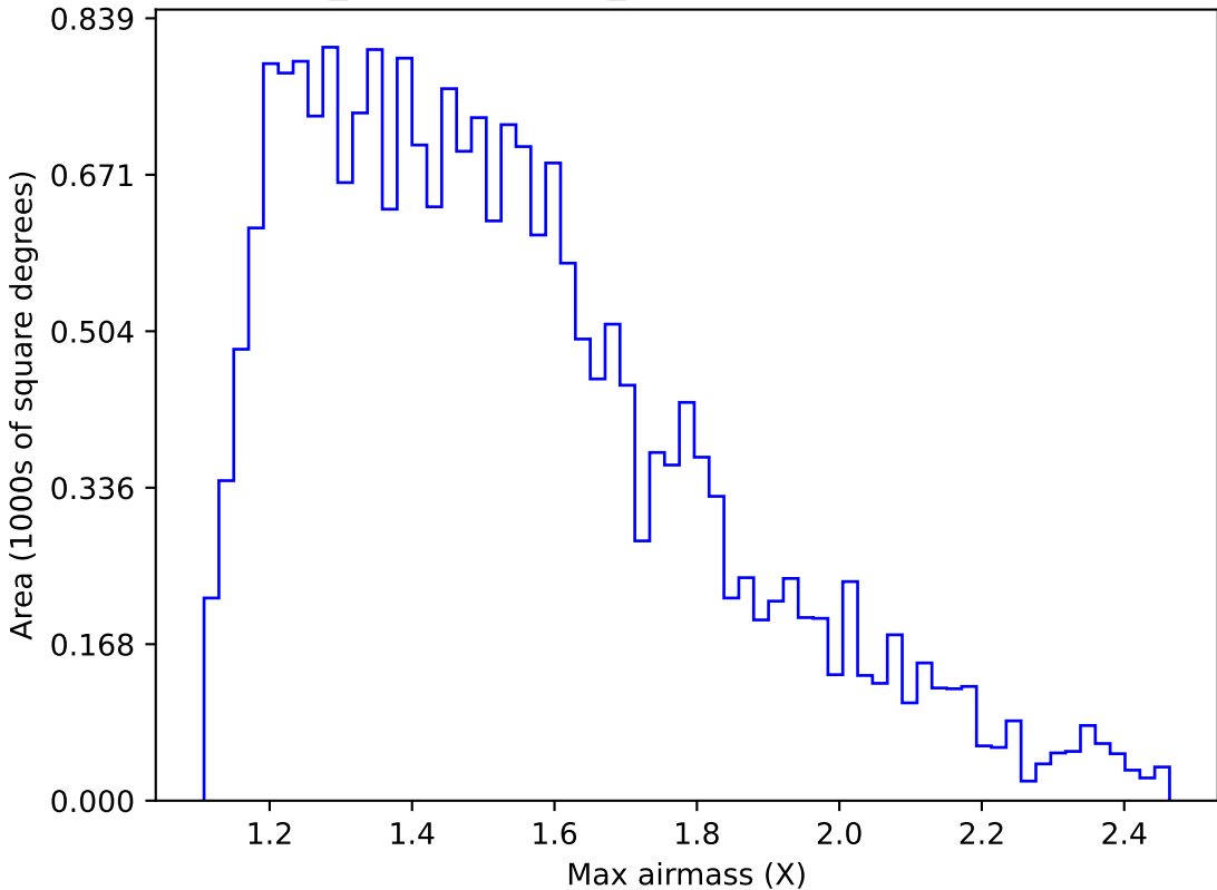
weather_cloudso36v3.4_10yrs Yr 1 u band: Max airmass
