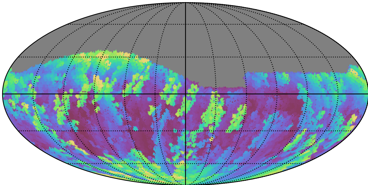
weather_cloudso36v3.4_10yrs Yr 1 r band: Max airmass
