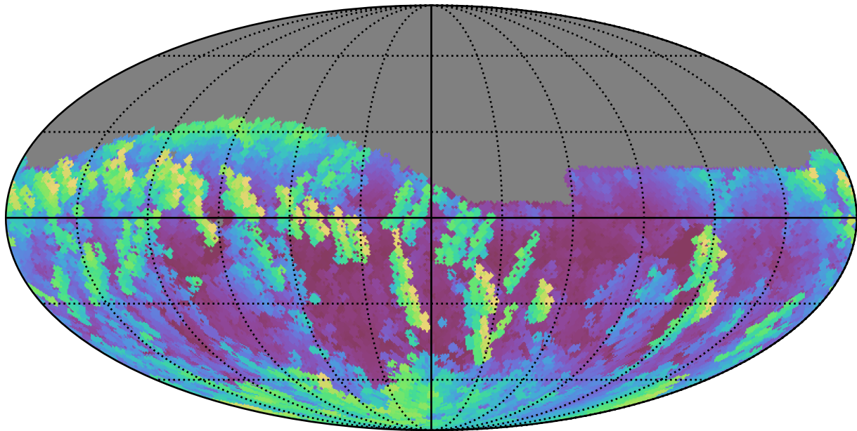
weather_cloudso36v3.4_10yrs Yr 1 i band: Max airmass
