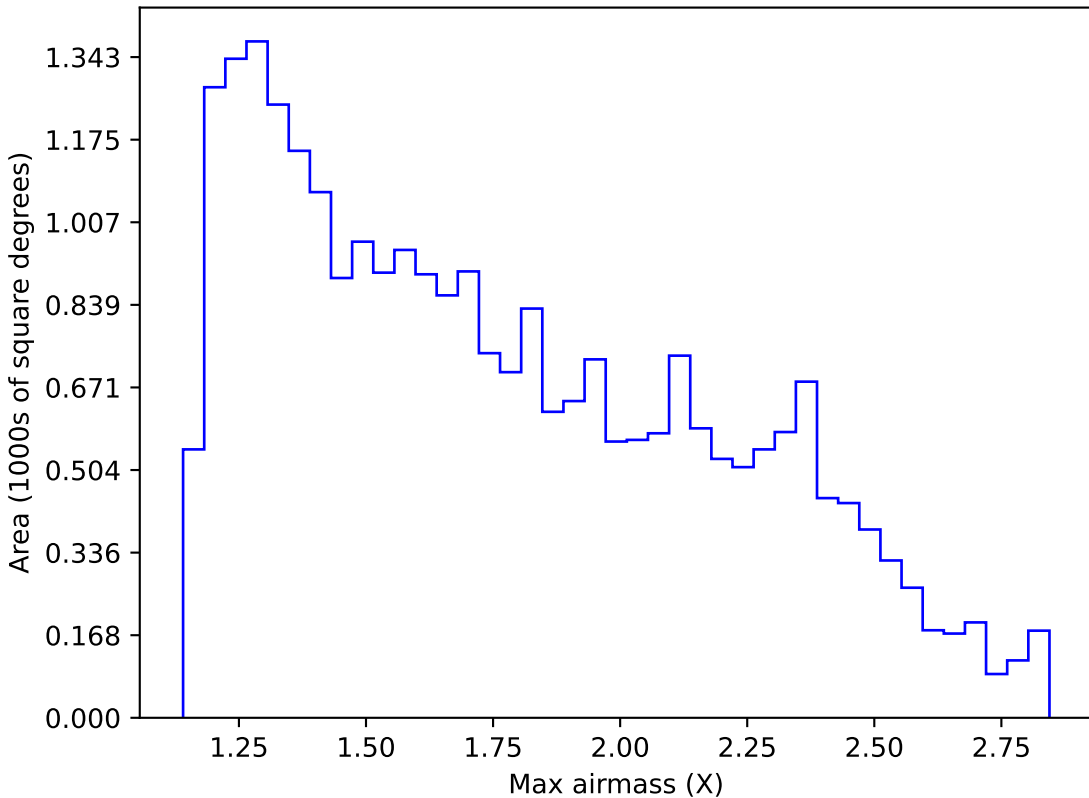
weather_cloudso36v3.4_10yrs Yr 1 i band: Max airmass
