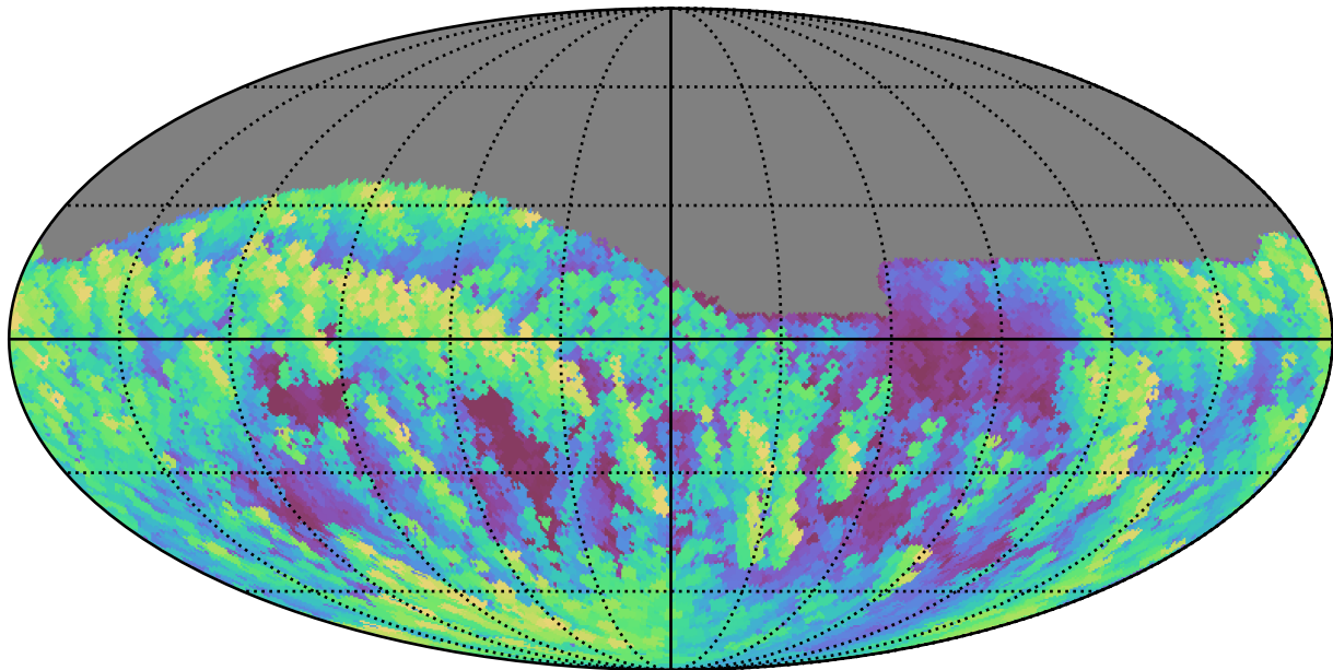
weather_cloudso36v3.4_10yrs Yr 1 all bands: Max airmass
