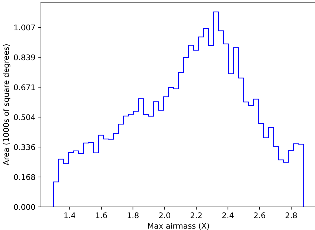
weather_cloudso36v3.4_10yrs Yr 1 all bands: Max airmass
