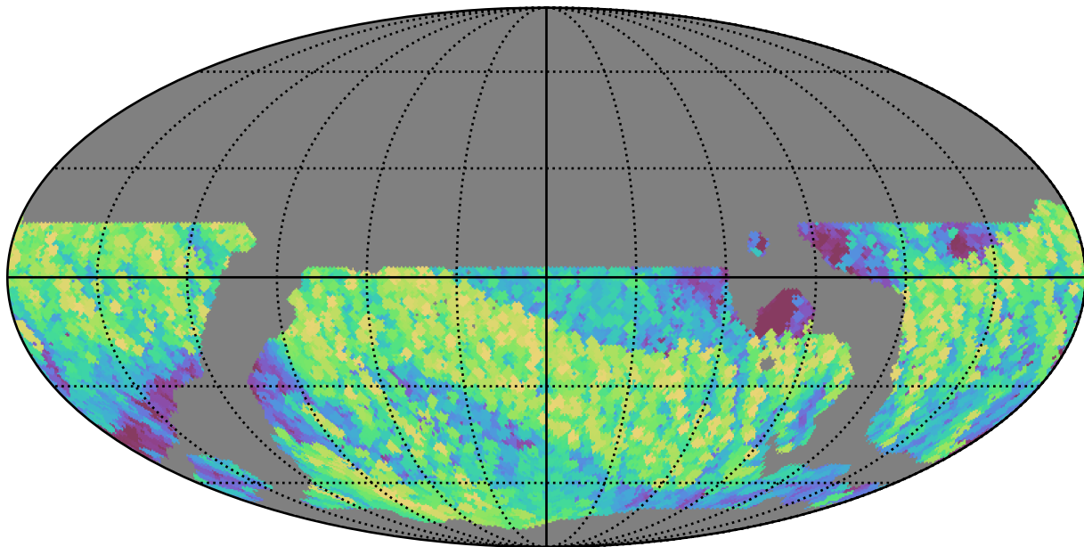
weather_cloudso36v3.4_10yrs WFD z band: Max airmass
