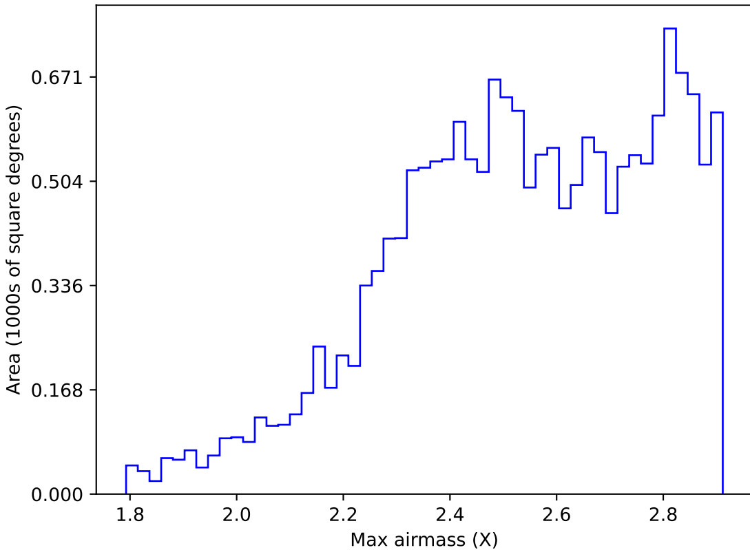
weather_cloudso36v3.4_10yrs WFD z band: Max airmass
