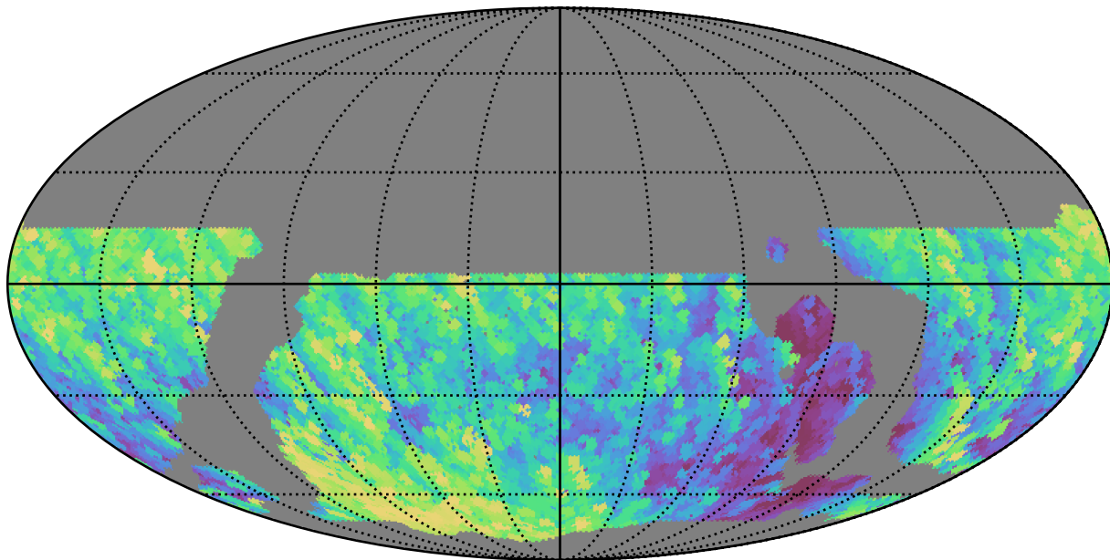
weather_cloudso36v3.4_10yrs WFD y band: Max airmass
