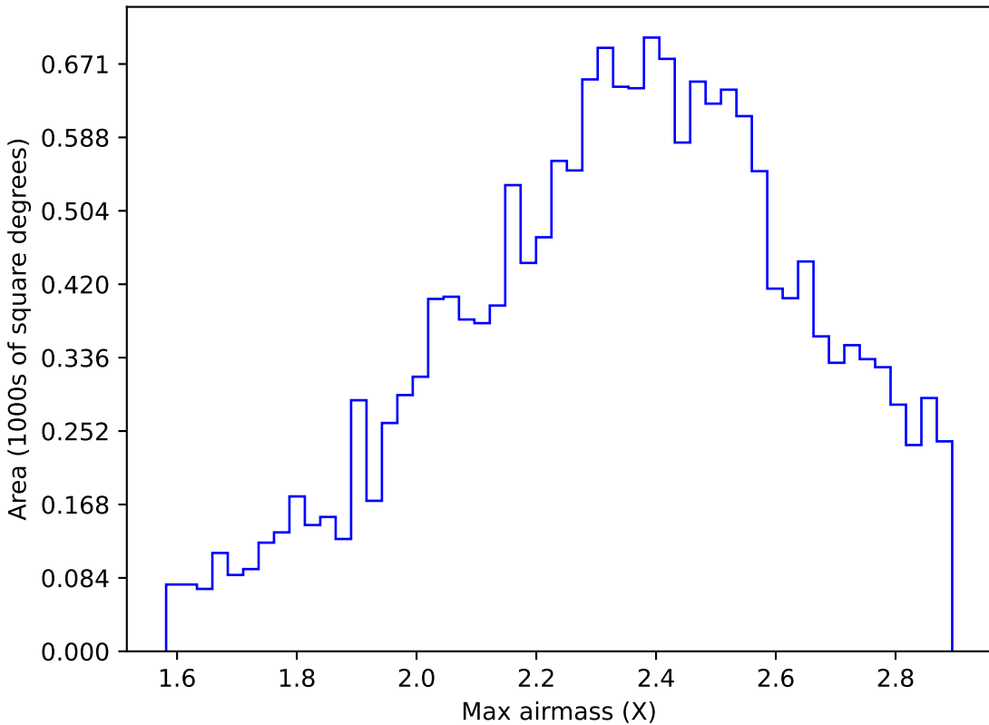
weather_cloudso36v3.4_10yrs WFD y band: Max airmass
