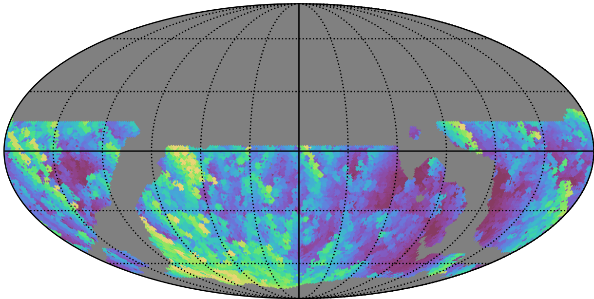
weather_cloudso36v3.4_10yrs WFD u band: Max airmass
